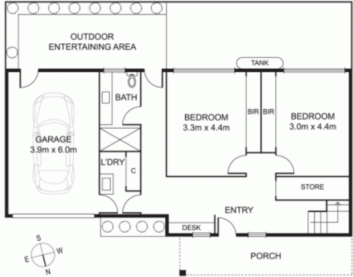
UPPER LEVEL
