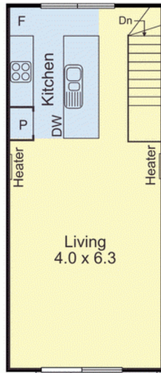
SECOND FLOOR
