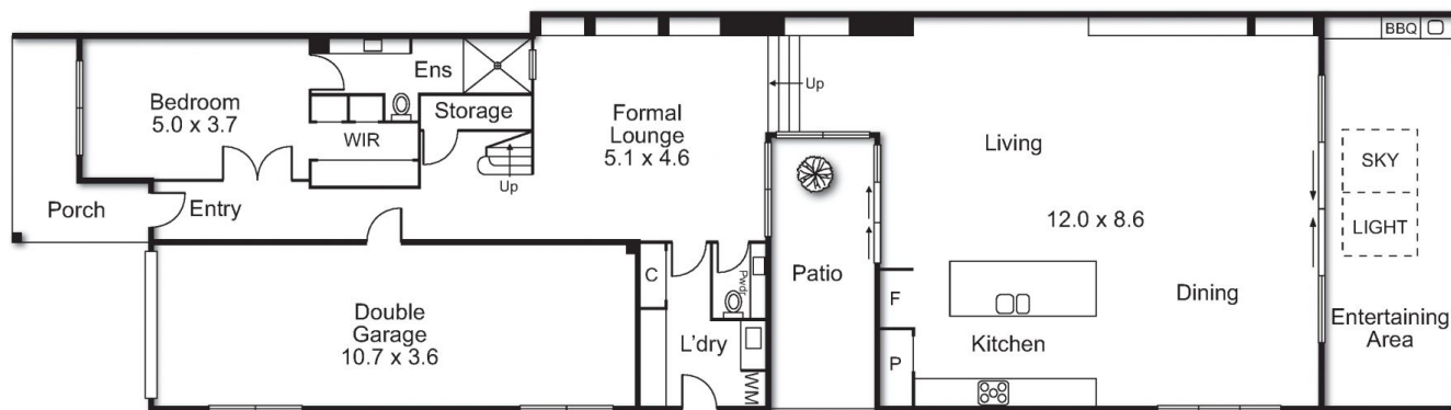
GROUND FLOOR
